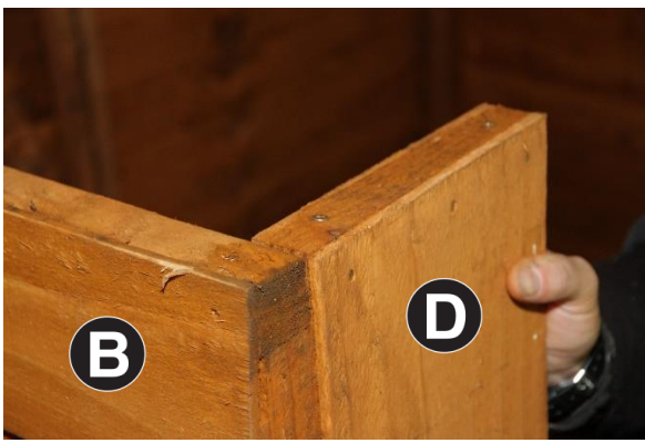
9. Ensure Panel D lines up with edge of Panel B framing leaving a 6mm overlap of the cladding as seen in image.
