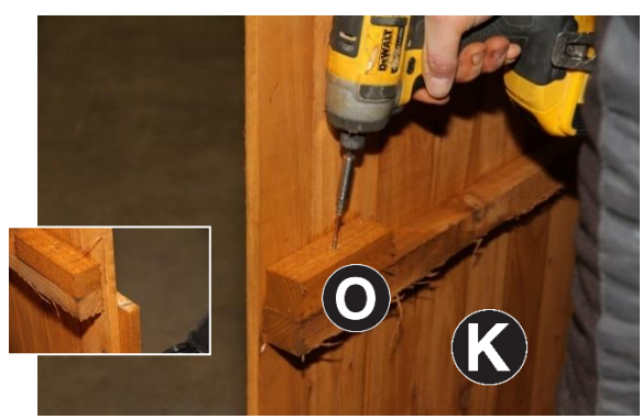
36. Fix Part O to Part K internal baton flush with Part K baton as shown in image using 2no 60mm screws. Repeat on opposite side door.
