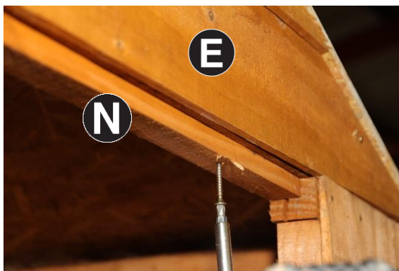
13. Attach Part N beneath Part E as shown using 4no 40mm screws.
