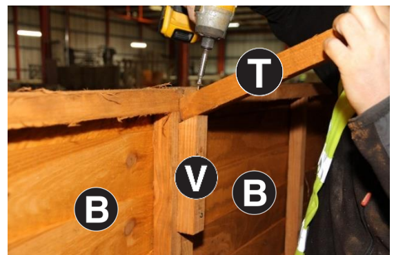
24. Fix Part T to Part V using 1no 60mm screw as shown in image.
