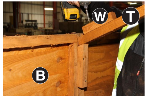
26. Attach Part W to Part T using 2no 60mm screws spaced evenly 40mm from end of Part T as shown on image. Repeat on both sides.
